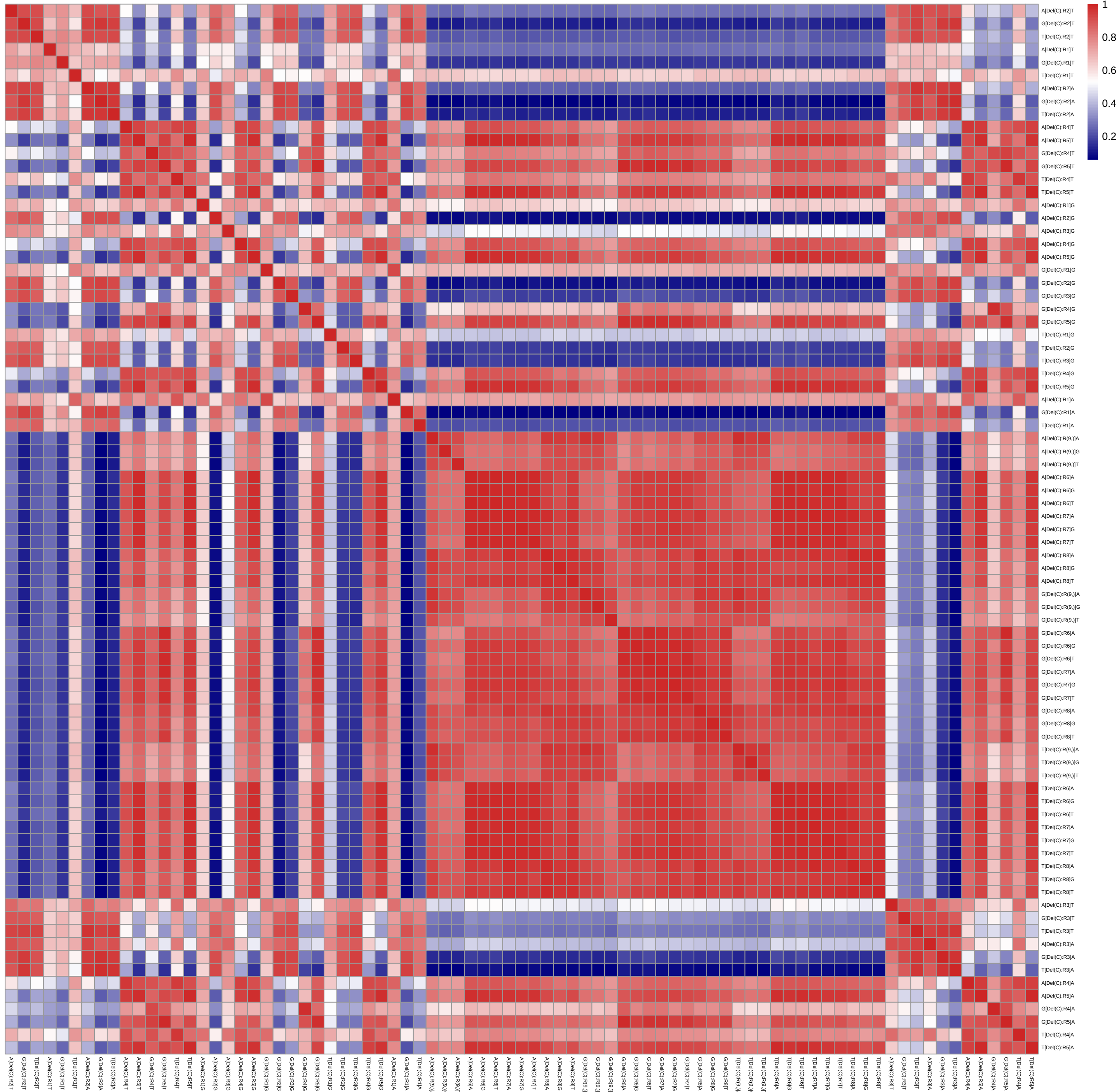
Heatmap (Strict ID89 Order) - Del_1bp_C
